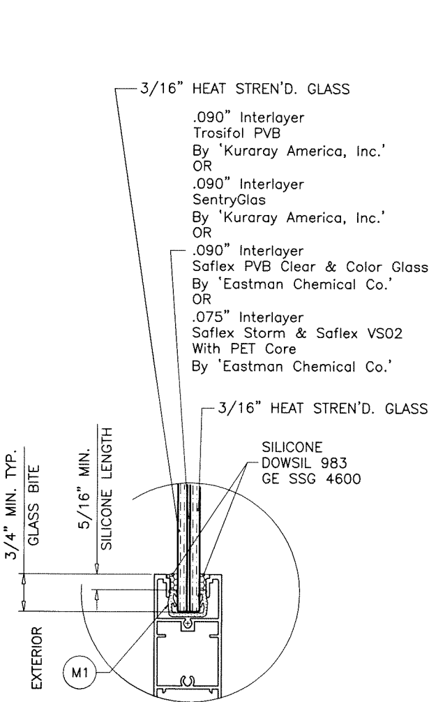
GLASS TYPE 'A' 7/16" OVERALL LAM. GLASS
