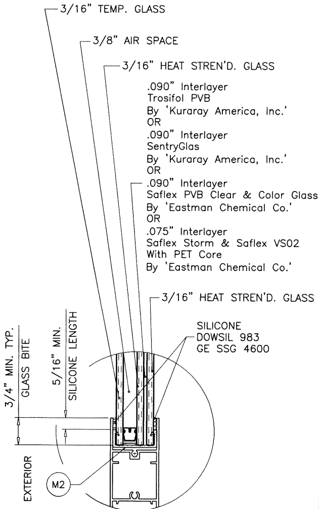
GLASS TYPE 'A1' 1" OVERALL INSUL. LAM. GLASS
