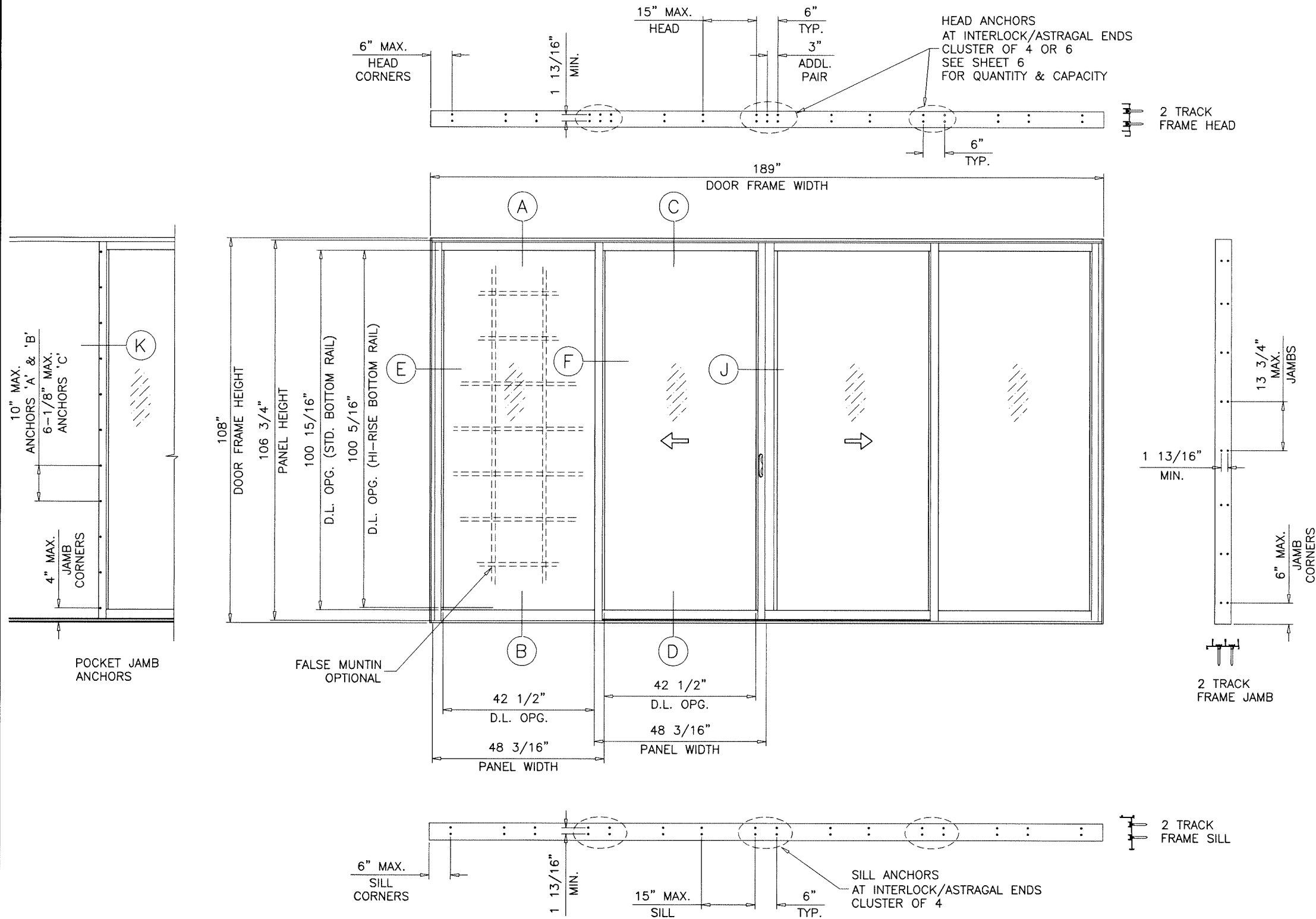
TYPICAL ELEVATION OX-XO
